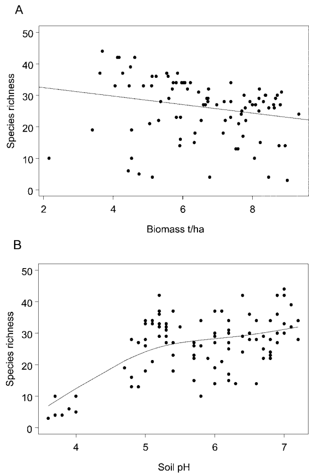
Figure 1: Correlates of whole-plot species richness, D_3 . A , Species richness declines with increasing biomass, as measured by long-term mean hay yield from the first cut in June (t ha -1 dry matter). B , Species increases nonlinearly with soil pH. The fitted line is a nonparametric smoother (cubic B-spline smooth, with df = 3.5 ). The nonlinearity is significant as assessed by the addition of a quadratic term for soil pH to a linear model ( t = -4.166 , df = 94 , P < .001 ). Each point represents one of the 97 plots.
